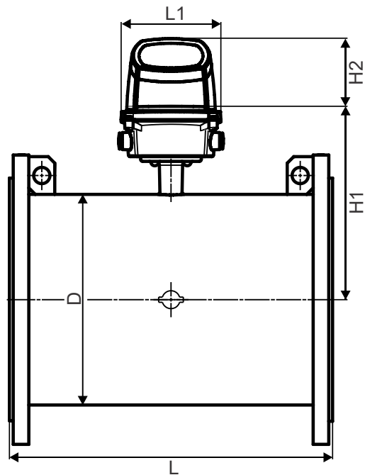
Flow sensor and transmitter
