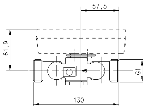
Mounting length 130 mm (threaded)
