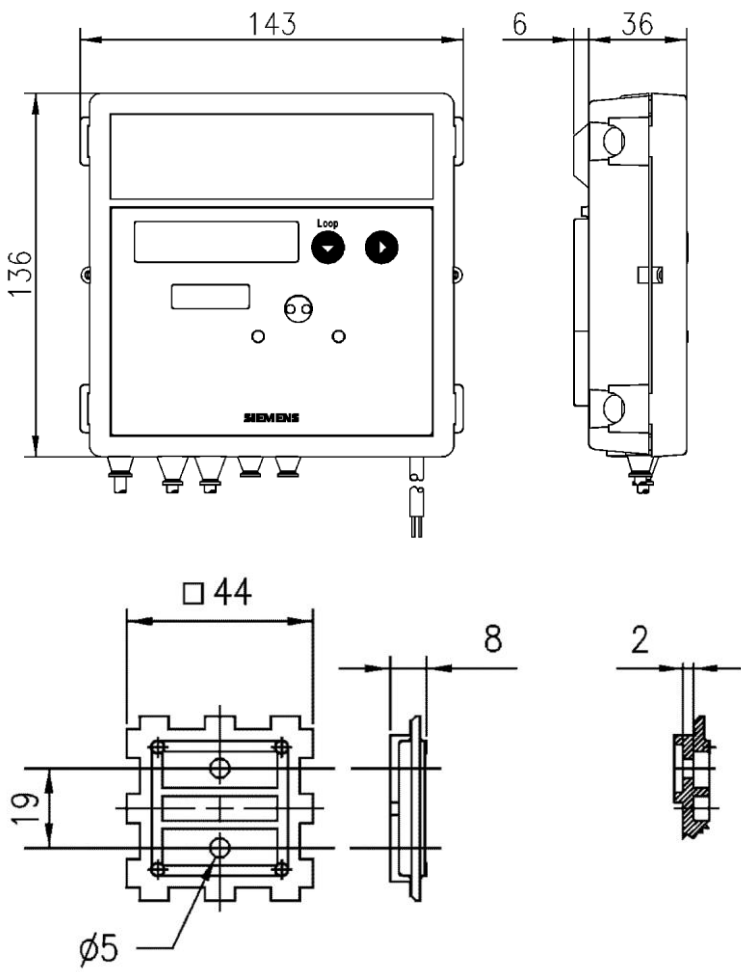
Adapter plate
