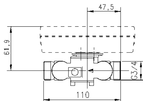
Mounting length 110 mm (threaded)
