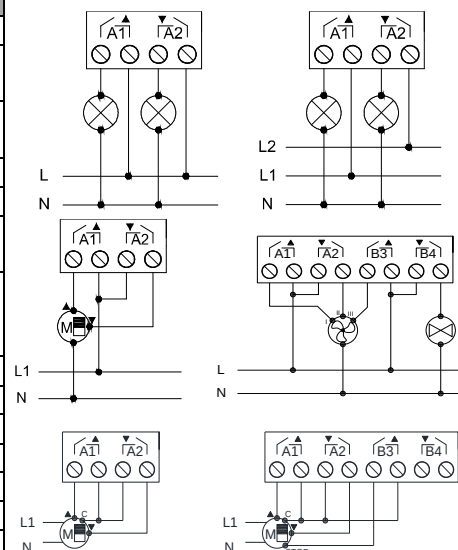
Figure 2: Wiring example (from left to right, and up to down): 2 loads, 2 loads connected to different phases, shutter, fan coil, shutter with 2 dry contacts, shutter with 3 dry contacts.
