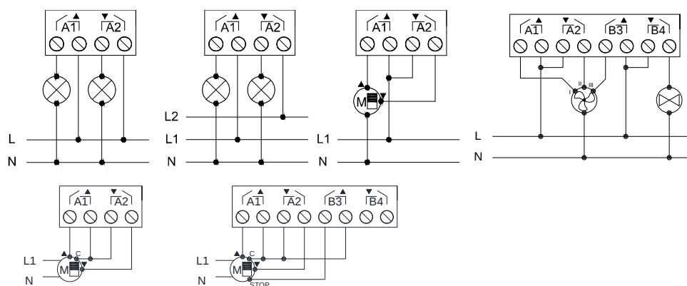
Figure 2: Wiring example (from left to right): 2 loads, 2 loads connected to different phases, shutter and fan coil, shutter with 2 dry contacts, shutter with 3 dry contacts.
