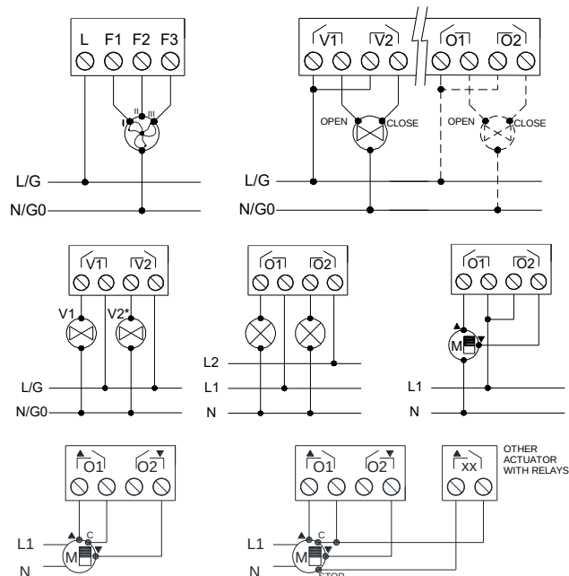
Figure 2: Wiring example (from left to right and from top to bottom): Three-speed fan, 1 or 2 three-point valves, 2 open/close valves, 2 loads connected to different phases, shutter channel, shutter with 2 dry contacts and shutter with 3 dry contacts
