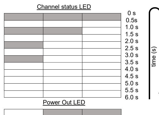
Figure 2: Error notification LED codes
