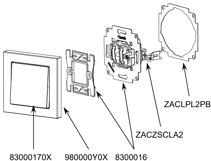
Figura 1. Interruptor simple
