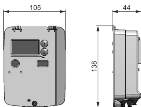
Fig. 5: Dimensions Processor
