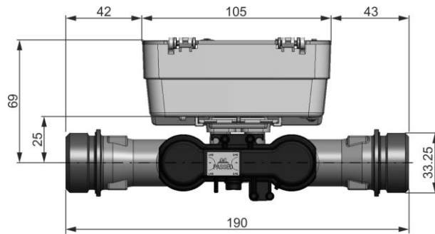
Fig. 9: Overview of dimensions mounting length 190 mm (threaded)
