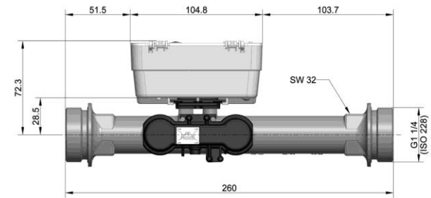
Fig. 10: Overview of dimensions mounting length 260 mm (threaded)
