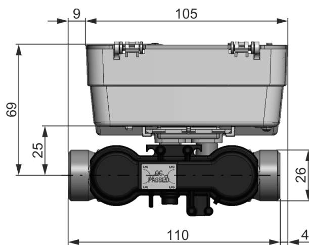
Fig. 7: Overview of dimensions mounting length 110 mm
