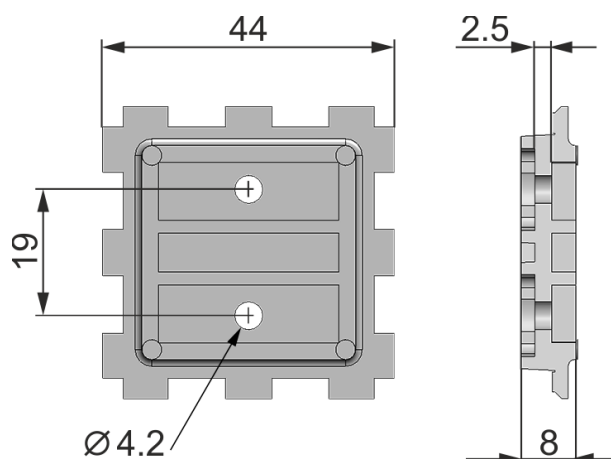
Fig. 6: Top view and cross section of the adapter plate
