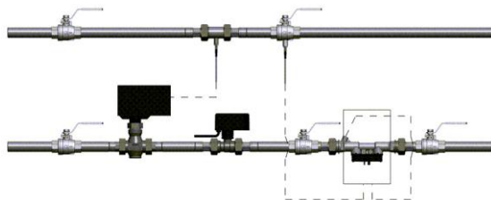
Fig. 3: Integration for circuit with e.g. throttling circuit (flow sensor in the direction of flow prior to control valve / differential pressure controller)
