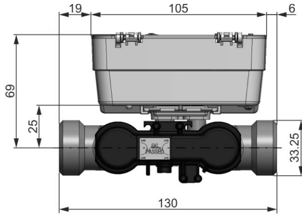
Fig. 8: Overview of dimensions mounting length 130 mm (threaded)
