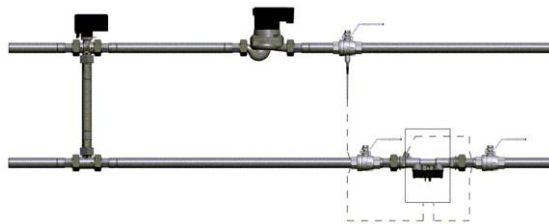
Fig. 2: Integration for circuits with mixing; placement of the temperature sensor
