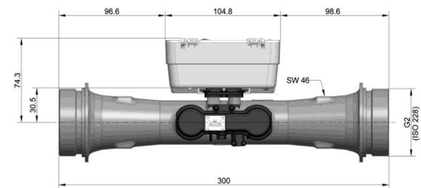
Fig. 11: Overview of dimensions mounting length 300 mm (threaded)
