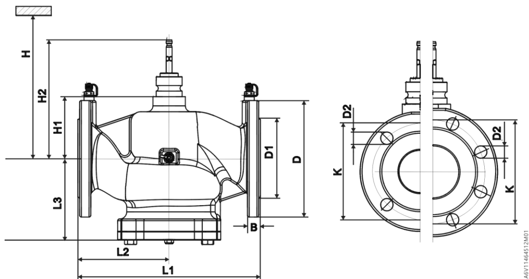
Dimensions in mm: VPF44../VPF54..
