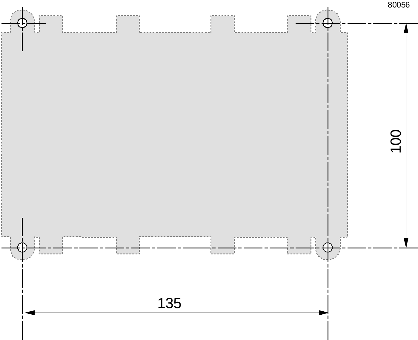
Drilling diagram 1:1
